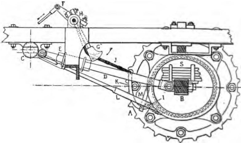
FIG. 382.—The Hub Brake and Operating Levers Used on the Panhard Carriages.—The arm, F, being pushed in the direction of the arrow, causes the arm, G, on the same pivot, H, to move in the opposite direction, as indicated by the lower arrow. Through this arm, G, runs the cable, J, as shown, which, pulling on the arm, K, pivoted at L, pulls the strap, shown by dotted lines around the drum, S. The other end of the strap attached to the short arm of the lever, K, is thus drawn toward the same point; a tight frictional bind being the result.
